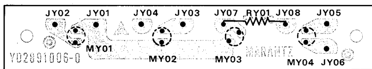
Figure 13. Indicator Lamps Assembly PY01 Component Locations
