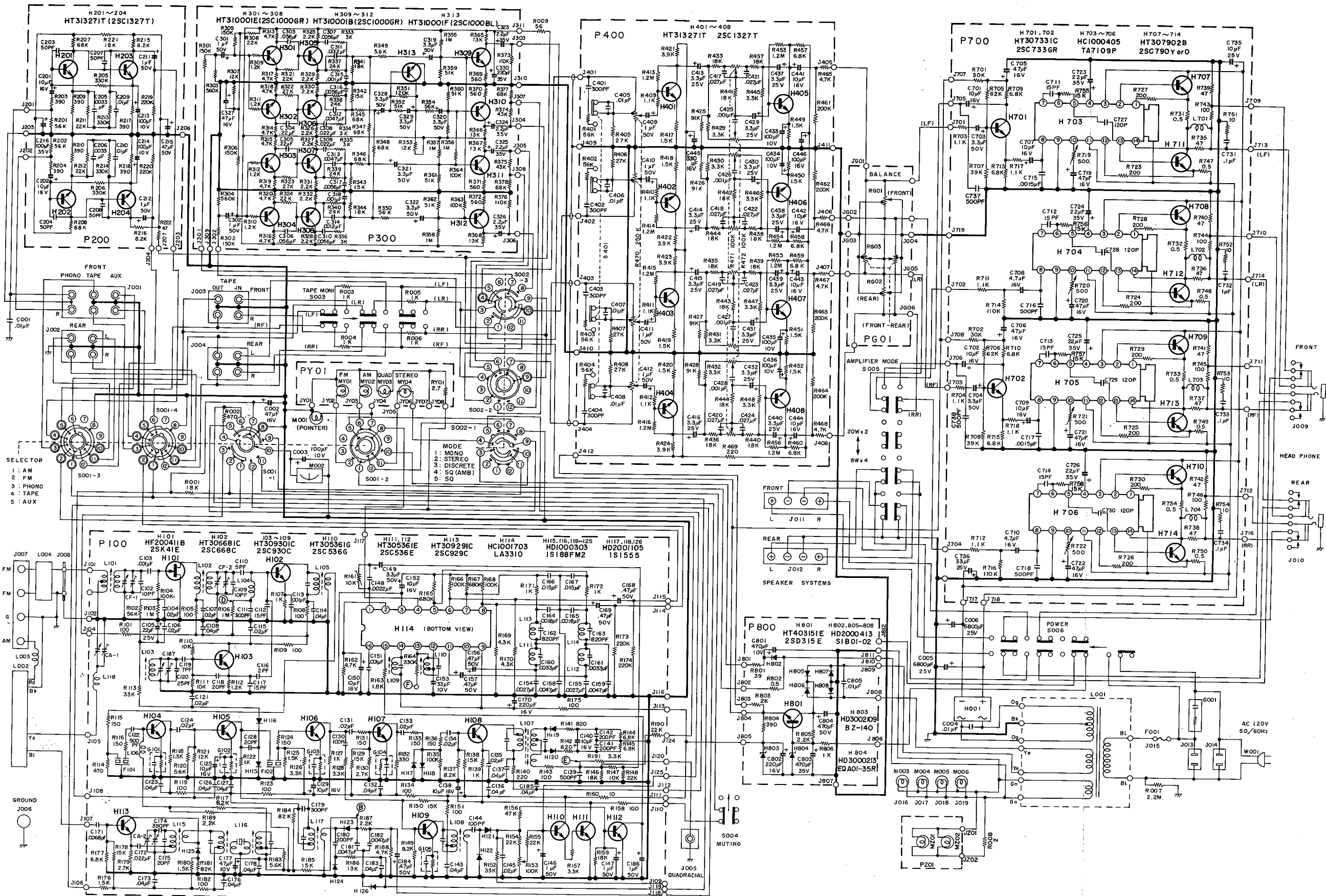
Figure 14. Schematic Diagram
