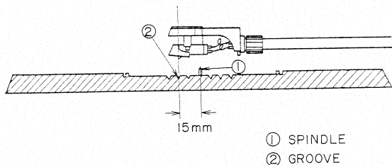
Fig. 14 Overhang Adjustment
