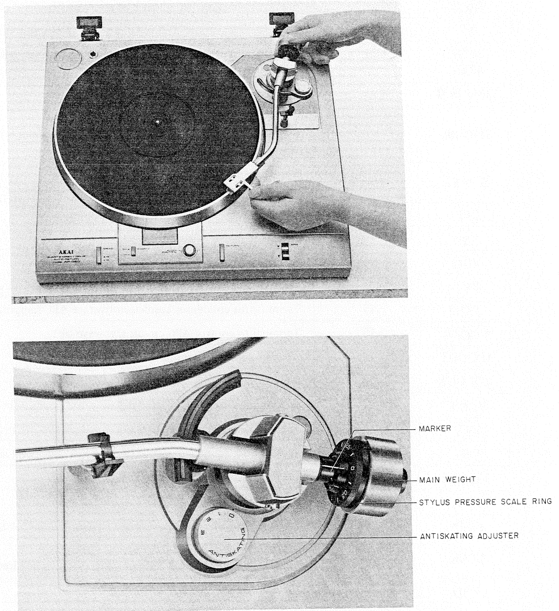
Fig. 13 Stylus Pressure Adjustment
